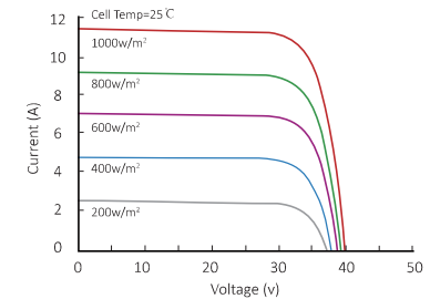
Current-Voltage Curve (LR4-60HPB-360M)
